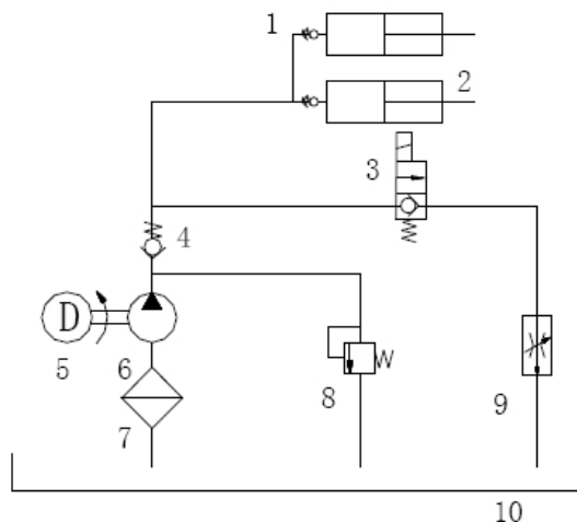
Fig.8 Principio della parte idraulica Fig.8 Principle of hydraulic part Fig.8 Principle of hydraulic part Abb.8 Prinzip der Hydraulik
